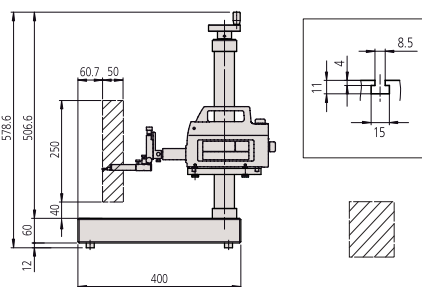
178-089 400x250x578 mm
