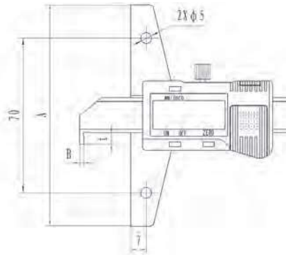
A = 100 mm B = 2 mm
