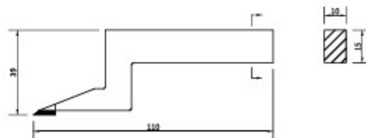
● 3130-4130 For:3130-8130 Range:0-1000/0-40" ● 3130-4130 For:3130-8135 Range:0-1500/0-60" ● 3130-4130 For:3130-8140 Range:0-2000/0-80"
