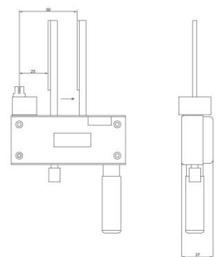
DIAMETER SHAFT FROM \varnothing 50 TO \varnothing 100 DIAMETRO ALBERI DA \varnothing 50 A \varnothing 100
